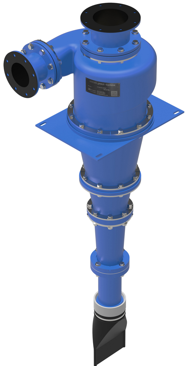
CycloStack boot installed on apex of cyclone to control the moisture in the coarse sand discharge
