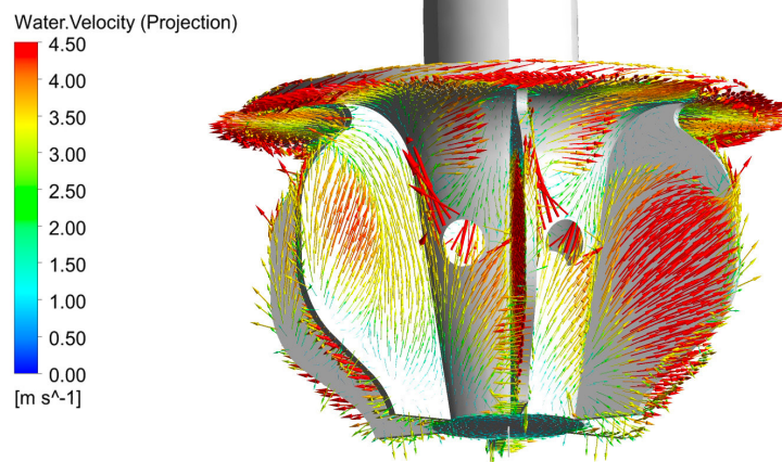
CFD illustrates the water velocities of the nextSTEP™ rotor are distributed over a wider area for more effective shear and bubble formation
